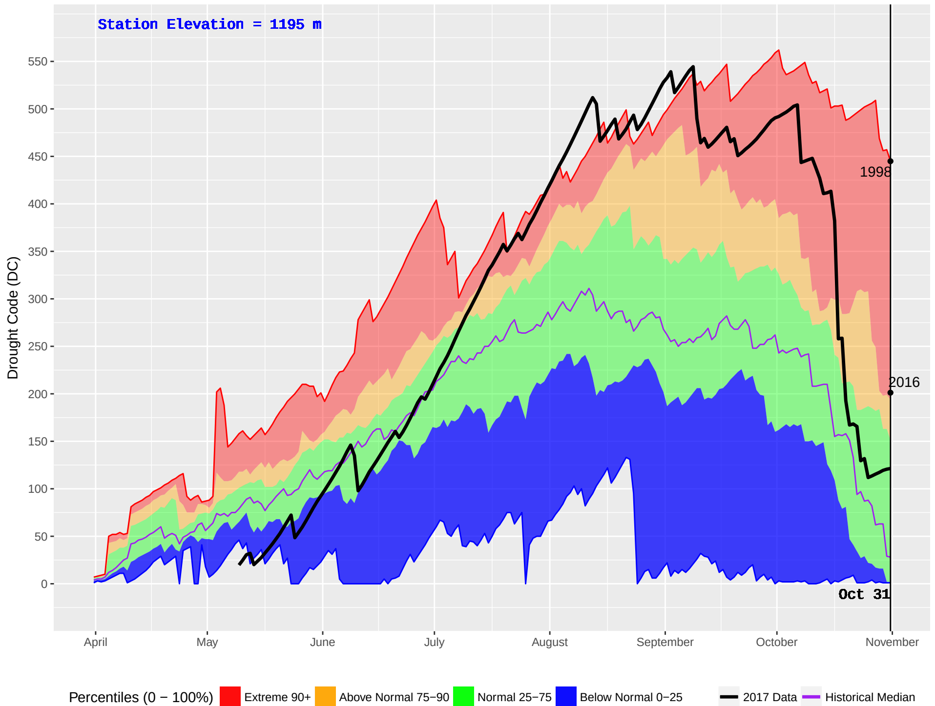
VALEMOUNT 2 (200) : Historical (1986–2016) and Current (2017) Noon Drought Code (DC)
