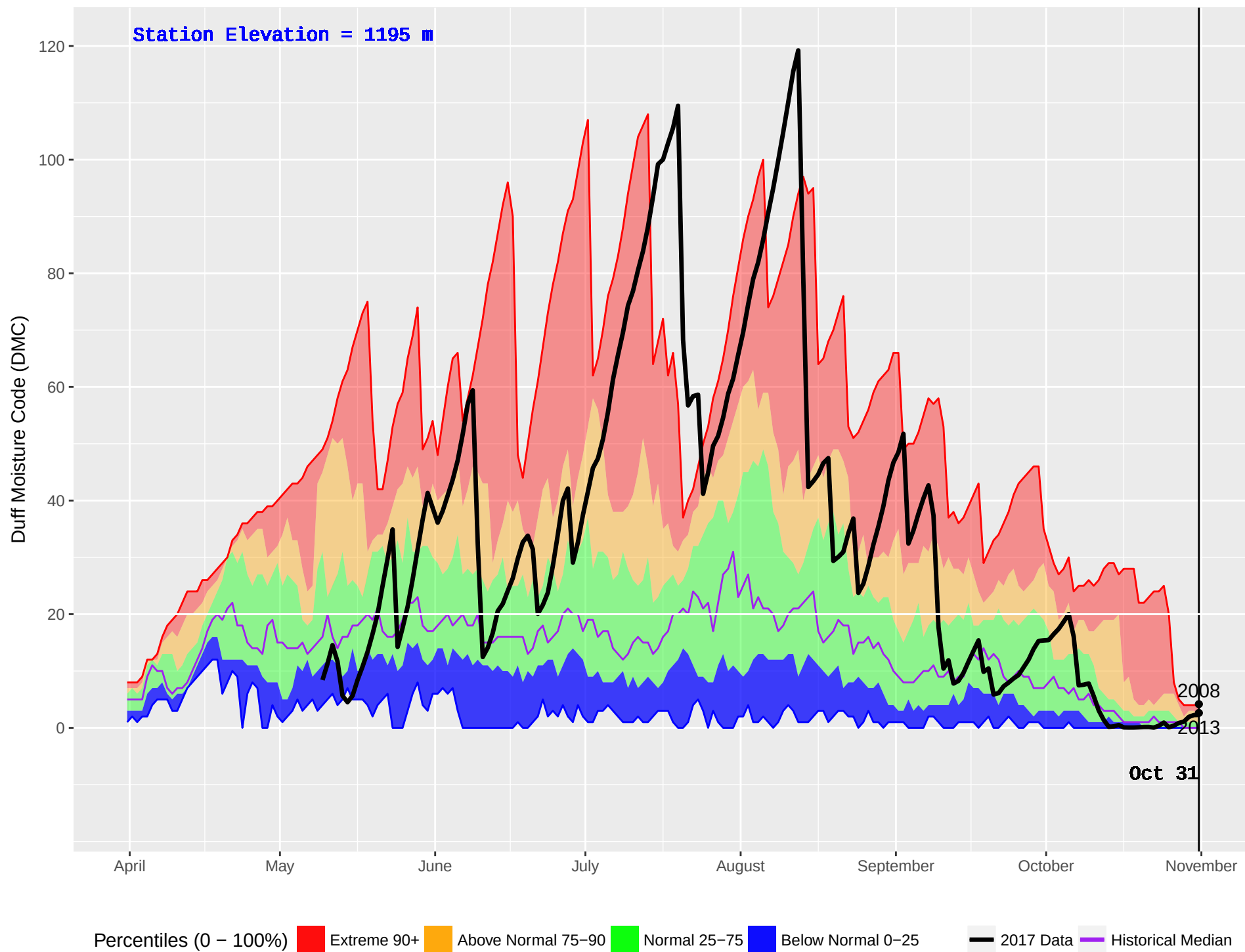
VALEMOUNT 2 (200) : Historical (1986–2016) and Current (2017) Noon Duff Moisture Code (DMC)
