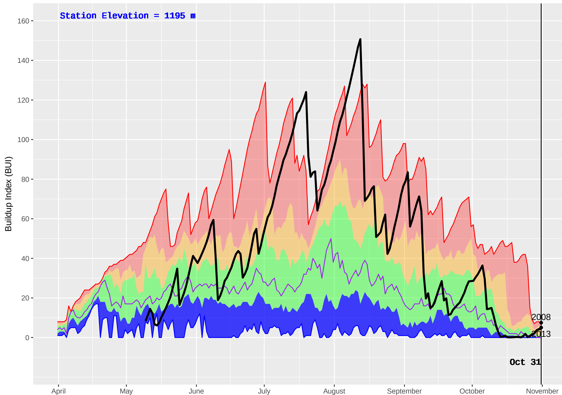
VALEMOUNT 2 (200) : Historical (1986–2016) and Current (2017) Noon Buildup Index (BUI)
